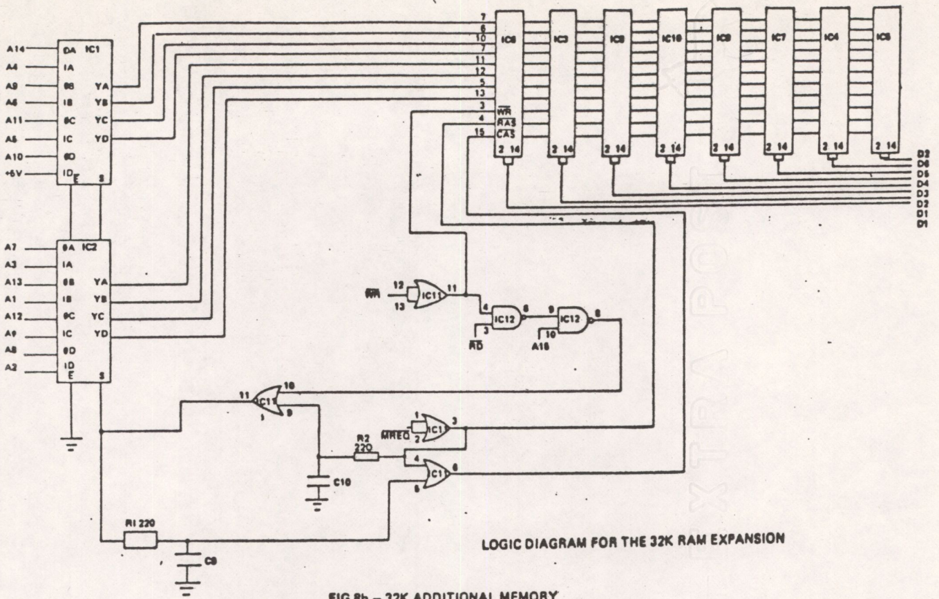
FIG 8b - 32K ADDITIONAL MEMORY
